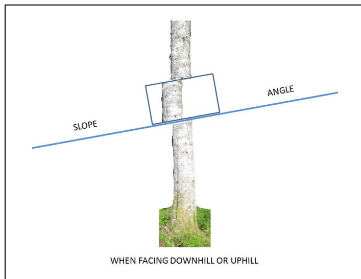
FIGURE 5: CORRECT POSITION OF PRISM ON SLOPES > 10%
